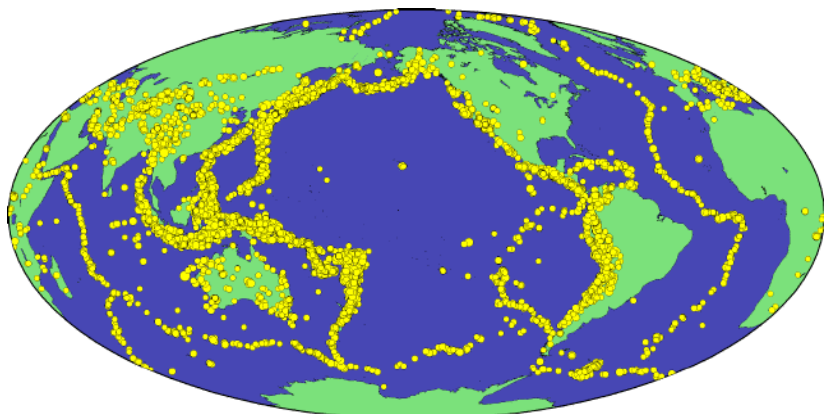
Figure 1: Distribution of earthquakes from 1900-1997 with magnitude greater than 5 (reprinted from [1]).
