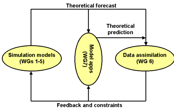
Figure 3. The ACES Science Plan involves a feedback process to ensure simulation models are developed which yield theoretical forecasts compatible with, and constrained, by the observed data. The theoretical forecasts are used to develop new applications or forecasting methods which are also refined through a similar feedback process.
