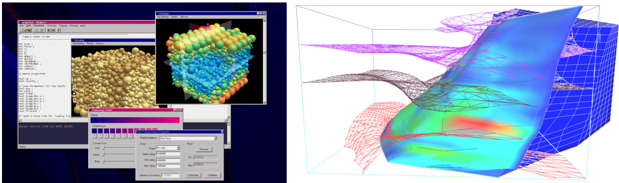
Figure 6: Left: The LSMearth micro-scale modelling software system developed at QUAKES showing a system of particles representing a rock structure being subjected to compression. Right: The GeoFEM macro-scale software system developed at RIST by the GeoFEM group showing a large scale simulation of a subduction fault zone.
