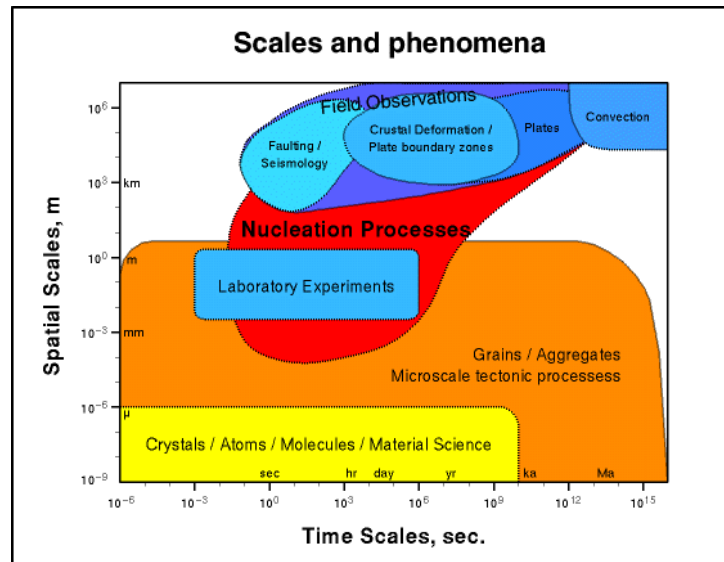
Figure 2: Scales and phenomena involved in the earthquake generation process (reprinted from [1]).
