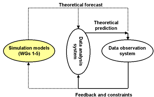
Figure 4. Illustration of how ACES adds to, and is complementary with, pre-existing earthquake prediction and/or hazard quantification programs and systems, which are based on data observation and analysis (shown in white).
