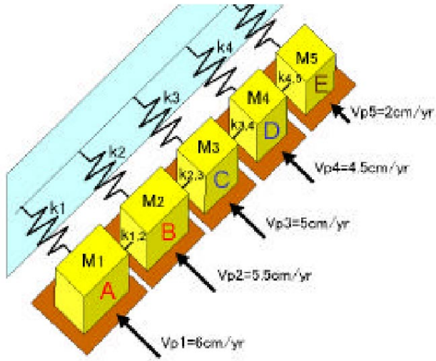
Figure 2: Block-spring model. Five blocks represent fault segments along the Nankai trough.
