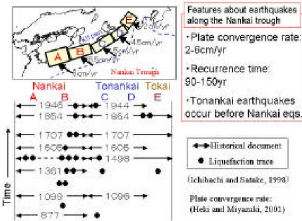
Figure 1: Space-time distribution of great earthquakes along the Nankai trough.
