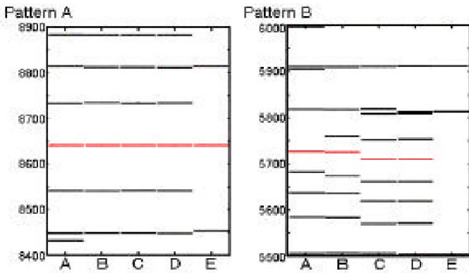
Figure 3: Block behavior patterns, showing the time of slip, for large stiffness values.
